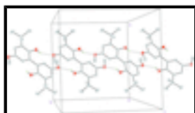
Fig. 2. The crystal packing of (I), showing hydrogen bonds as dashed lines along b axis. H atoms on C atoms have been omitted.
